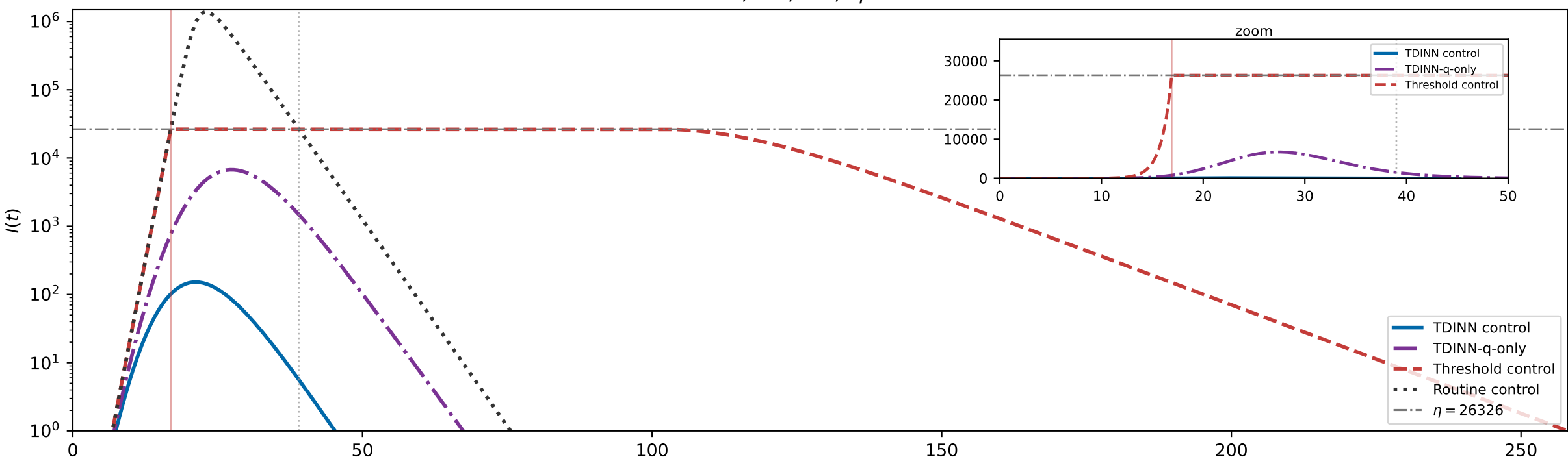
Daily new community infections
