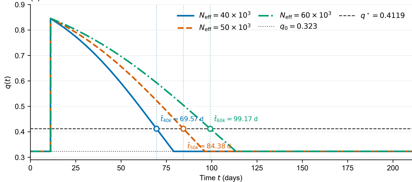
(b) Quarantine control and inflection times
