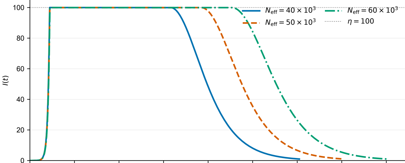
(b) Quarantine control and inflection times
