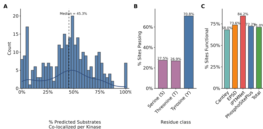
Figure 2: Cantley Atlas Filtering Results. A) Distribution of subcellular co-localization percentages for predicted kinase-substrate pairs per kinase. Co-localization was determined using Human Protein Atlas (HPA) subcellular location data, requiring at least one shared compartment between the kinase and substrate. The dashed line indicates the median co-localization (45.3%). B) Percentage of predicted sites passing filtering criteria across residue classes (Serine, Threonine, and Tyrosine). “Pass” is defined as a site being either previously curated in primary databases (PhosphoSitePlus, EPSPD, iPTMNet) or possessing a high functional score (Ochoa score >0.5). C) Comparative analysis of the percentage of functional sites across different data sources, highlighting the functional density of the predicted atlas relative to curated repositories.
