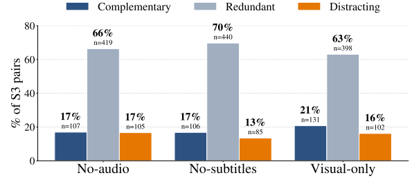
Figure 3: Share of S3 video pairs ( n=631 ) in each modality role (Complementary, Redundant, Distracting; defined in §4.4) for the three ablations. The mIoU change \Delta is averaged across three models before binning. Complementary and Distracting shares are roughly balanced and cancel in the mean mIoU.
