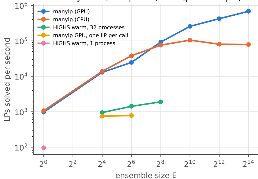
Community dFBA, 12 species, 48 h (pFBA-unique)
