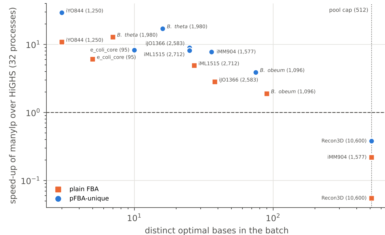
Genome-scale models, 1,024 members (reactions in brackets)
