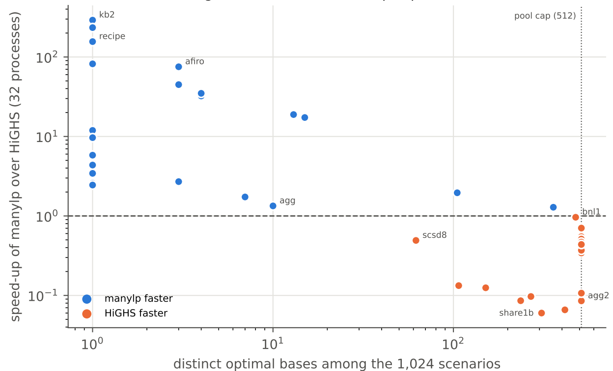
Netlib LPs, 1,024 right-hand-side scenarios per problem
