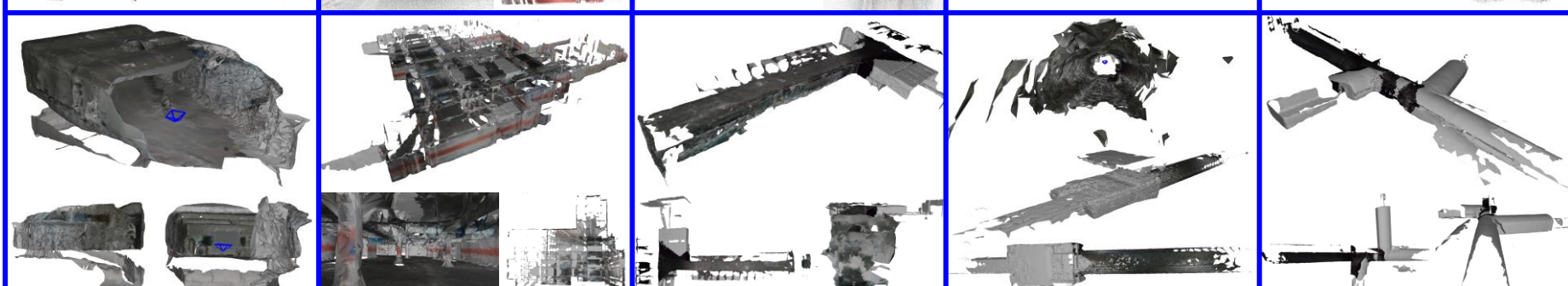
Ground- Fusion++
