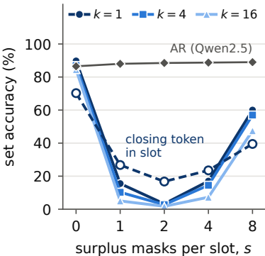
(a) Dream
