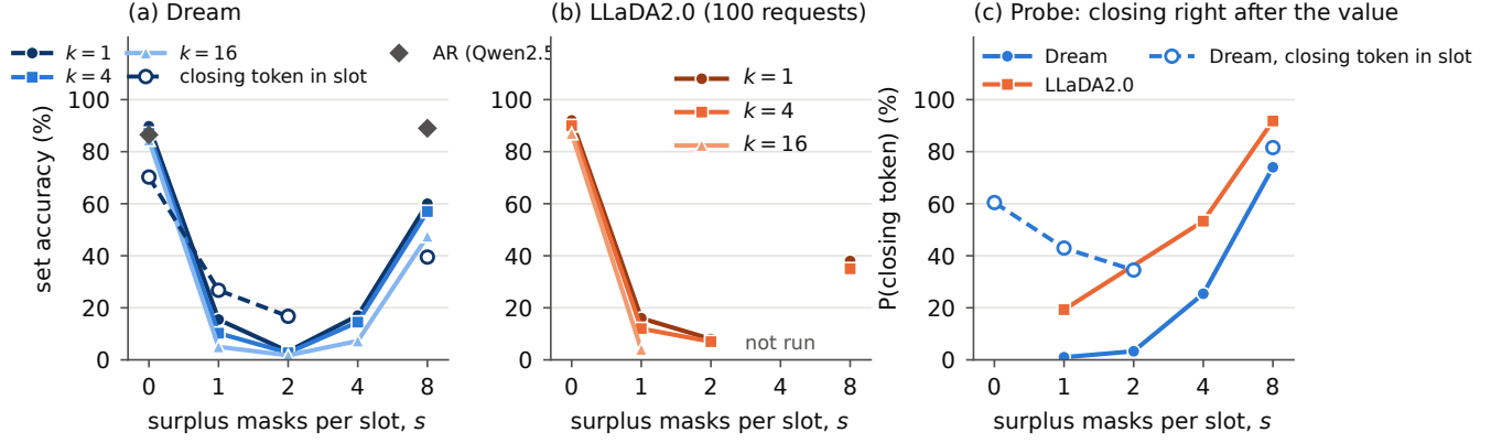
Figure 2: Every slot gets s masks more than its reference value has tokens. (a, b) Set accuracy against the surplus s , one line per k (tokens committed per step); LLaDA2.0 on its 100-request subset, where s = 4 was not run and k = 16 only up to s = 1 . Dashed: Dream at k = 1 with the closing token in the slot ( s = 4 not run). The AR agent stops at its closing token, so surplus masks only lift its cut-off. (c) Teacher-forced probe over all 3,063 slots: with the reference value written into the slot and s masks left before the skeleton’s closing delimiter, the mean probability that the next token closes the value. Dashed: with the closing token in the slot, where 1 + s positions remain.
