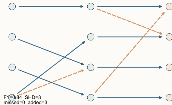
Schelling — Structured + bootstrap
