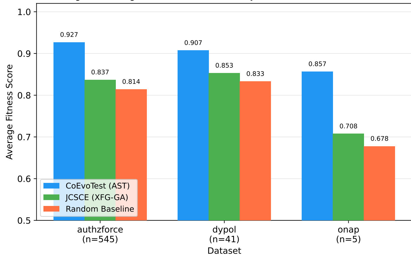
Fig. 1 - Average Fitness: CoEvoTest vs. JCSCE vs. Random Baseline
