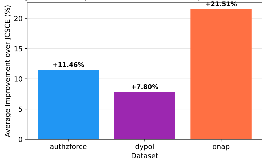
Fig. 3 - Fitness Improvement of CoEvoTest over JCSCE Baseline (%)
