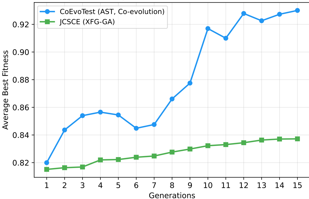
Fig. 5 - Convergence Curves (Fitness vs. Generations)
