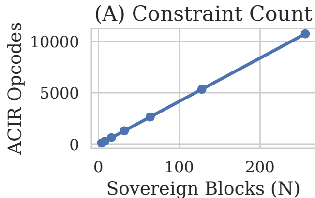
Figure 6 -- Recovery Proof Scaling (Noir + UltraHonk, real measurement)
