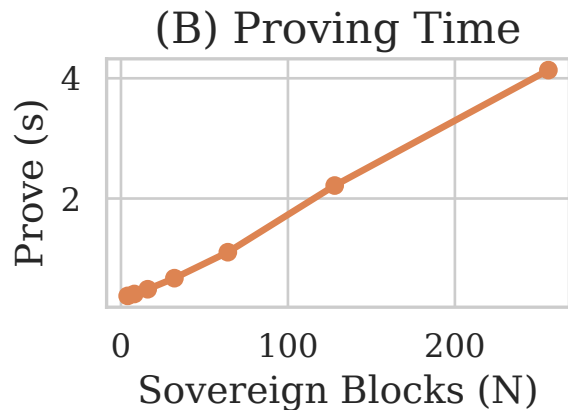
Figure 6 -- Recovery Proof Scaling (Noir + UltraHonk, real measurement)
