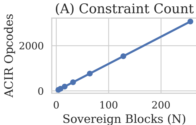
Figure 6 -- Recovery Proof Scaling (Noir + UltraHonk, real measurement)
