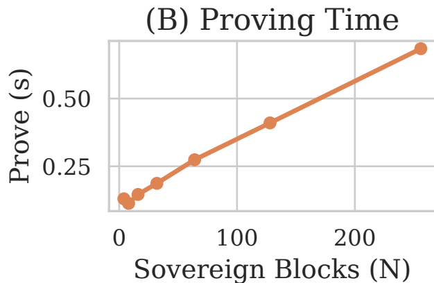
Figure 6 -- Recovery Proof Scaling (Noir + UltraHonk, real measurement)
