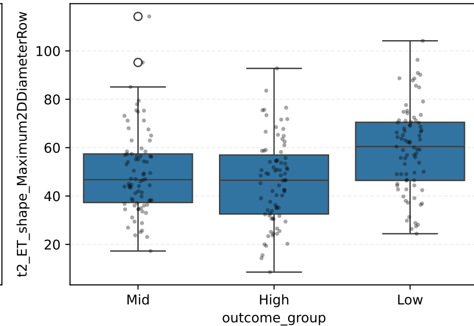
t2_ET_shape_Maximum2DDiameterRow
