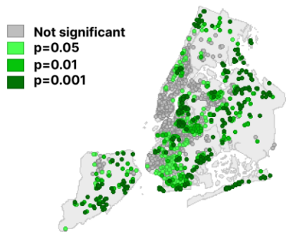
LISA significance map of NO
