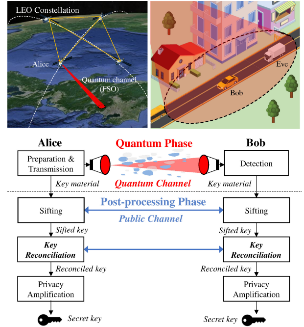
Fig. 1. LEO satellite-based FSO/QKD system for secure IoV applications and the block diagram of QKD protocols.
