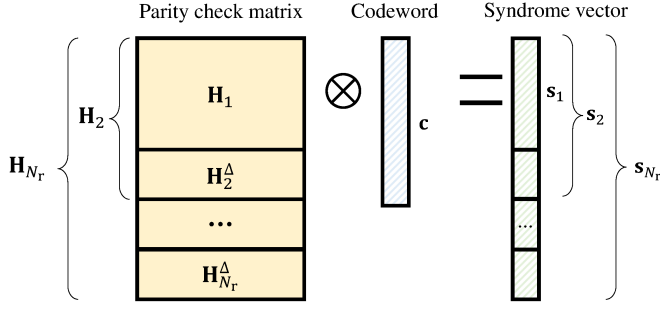
Fig. 5. Illustration of the proposed RC-LDPC code family and how created syndrome vectors can be nested.
