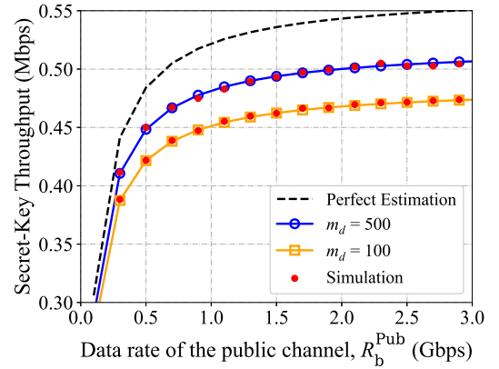
Fig. 11. Throughput versus the data rate of the public channel with different numbers of syndrome bits considered for error estimation, m_d .
