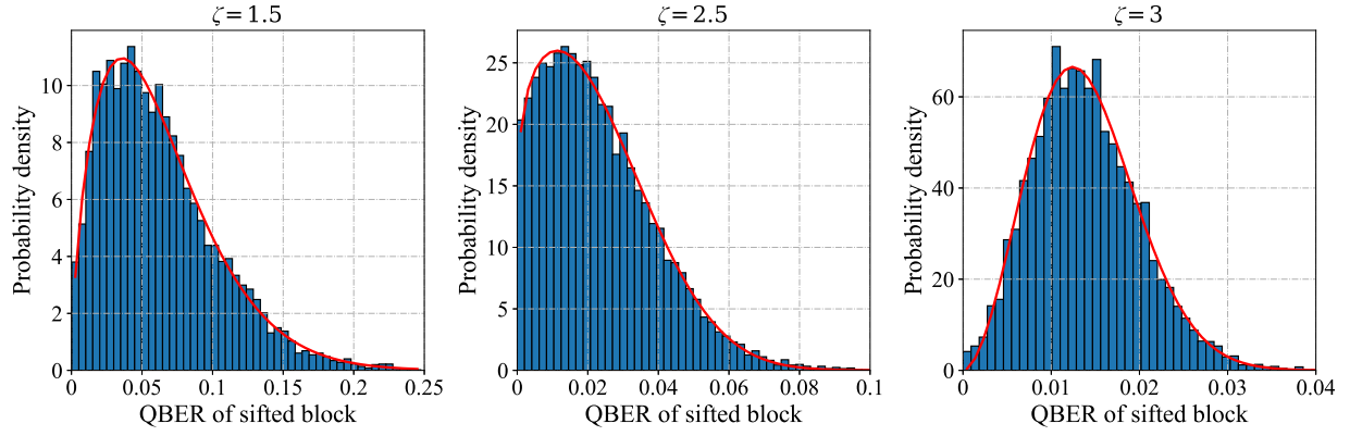
Fig. 8. Examples of simulation data histograms for sifted blocks' QBER and the fitting curves of the EB distribution with different DT scale coefficients, \zeta .
