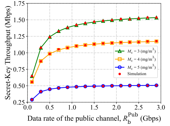
Fig. 10. Throughput of the proposed design versus the data rate of the public channel with different CLWC values, M_c .
