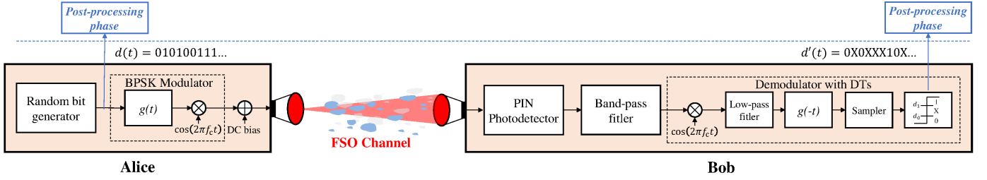
Fig. 3. Block diagram of the free-space CV-QKD protocol using SIM/BPSK and a dual-threshold detector implemented on the quantum phase.
