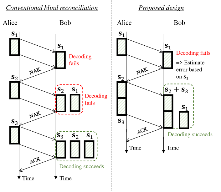
Fig. 4. The operations of the conventional blind reconciliation and the proposed design.
