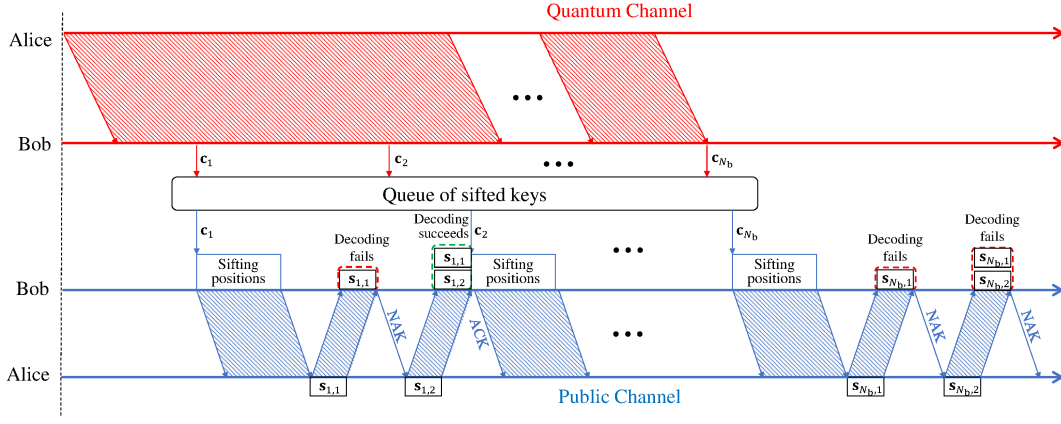
Fig. 2. An example of a superframe of the considered system, where the quantum phase is conducted via the quantum channel and the post-processing phase is conducted via the public channel.
