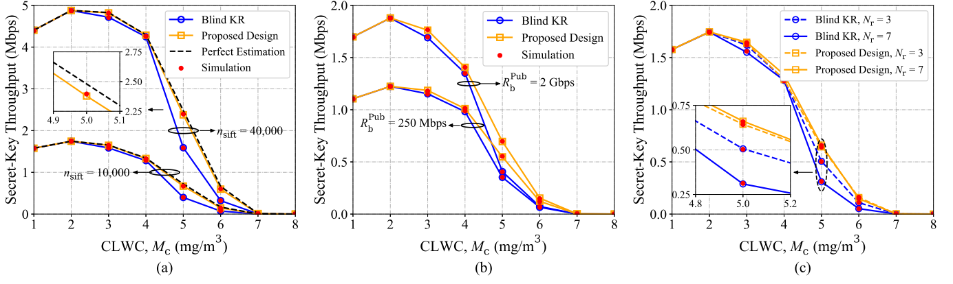
Fig. 9. SKT performance of the proposed design and the blind reconciliation versus CLWC with different (a) block lengths, n_{\text{sift}} , (b) data rates of the public channel R_b^{\text{Pub}} , and (c) maximum number of code rates in the RC-LDPC code family, N_r .
