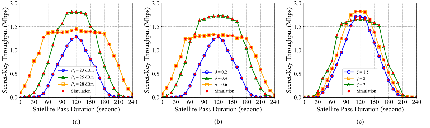
Fig. 12. Throughput performance over the satellite pass with different (a) LEO transmitted power, P_t , (b) modulation depths, \delta , and (c) DT scale coefficients, \zeta .
