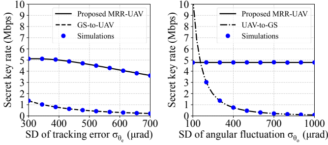
Fig. 2. SKR performance comparison under (a) GS tracking errors and (b) UAV hovering-induced angular fluctuations. The proposed MRR-UAV system outperforms the benchmark schemes in terms of robustness and SKR.
