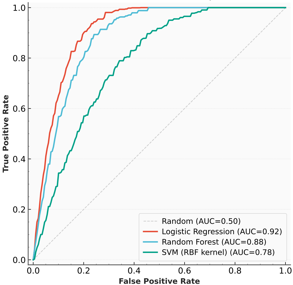
ROC Curves — Classifier Comparison
