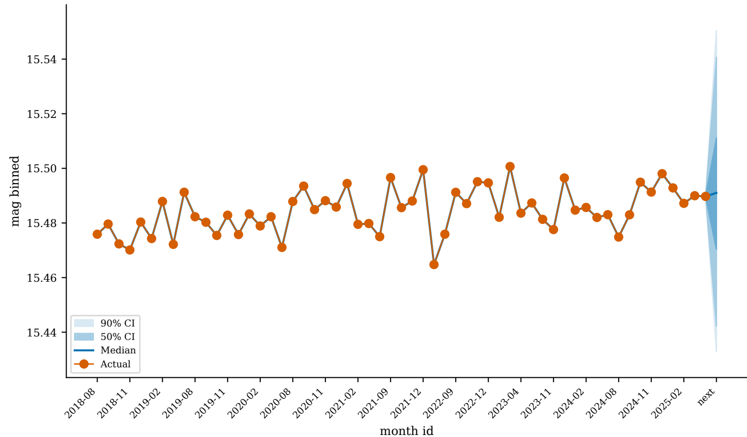
GaiaDR3_3333971597632801920 (high_uncertainty)
