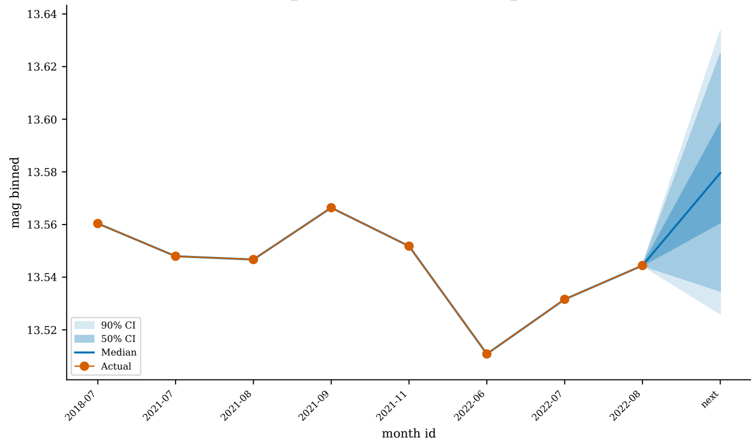
GaiaDR3_6898255177217741952 (worst_predicted)
