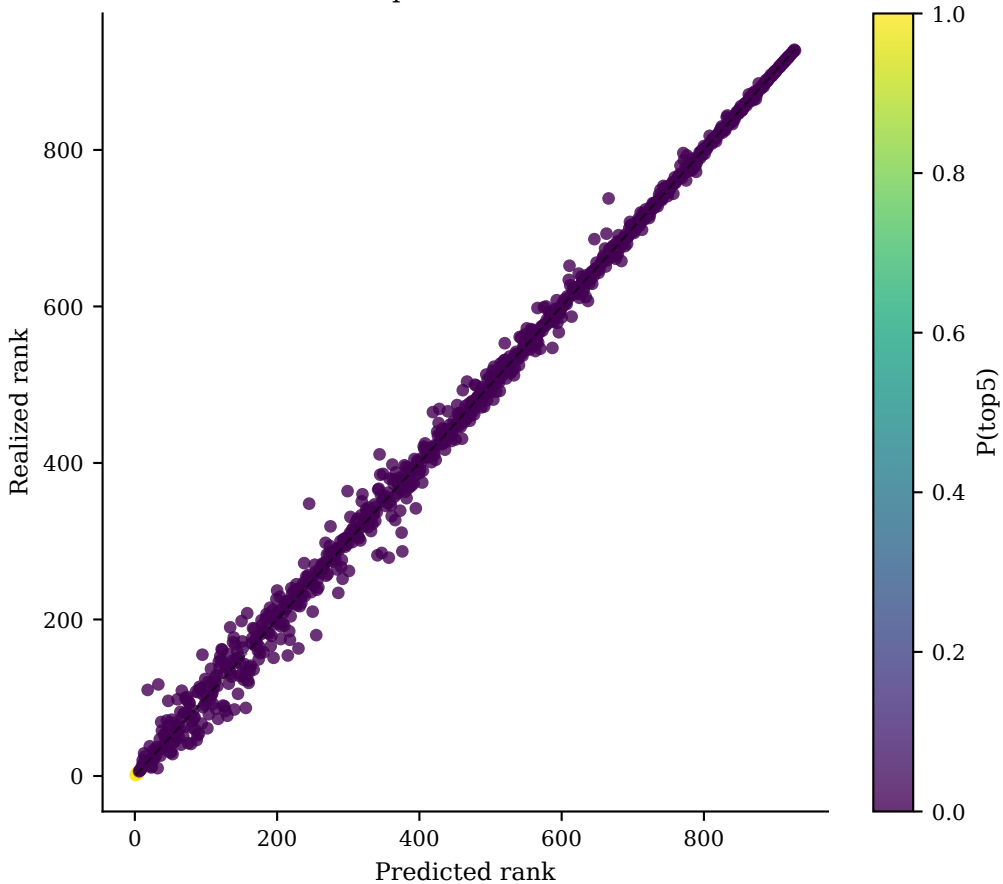
Held-out slate: predicted vs realized rank
