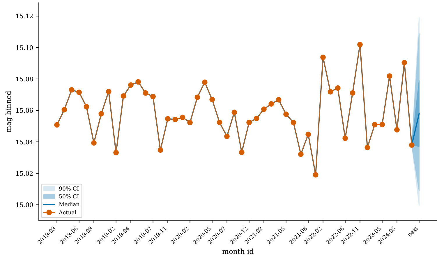
GaiaDR3_1445074014829920000 (worst_predicted)
