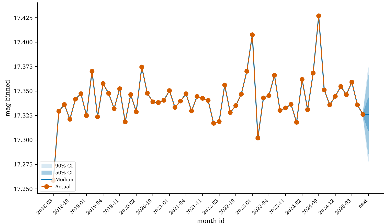
GaiaDR3_3108255943655246976 (best_predicted)
