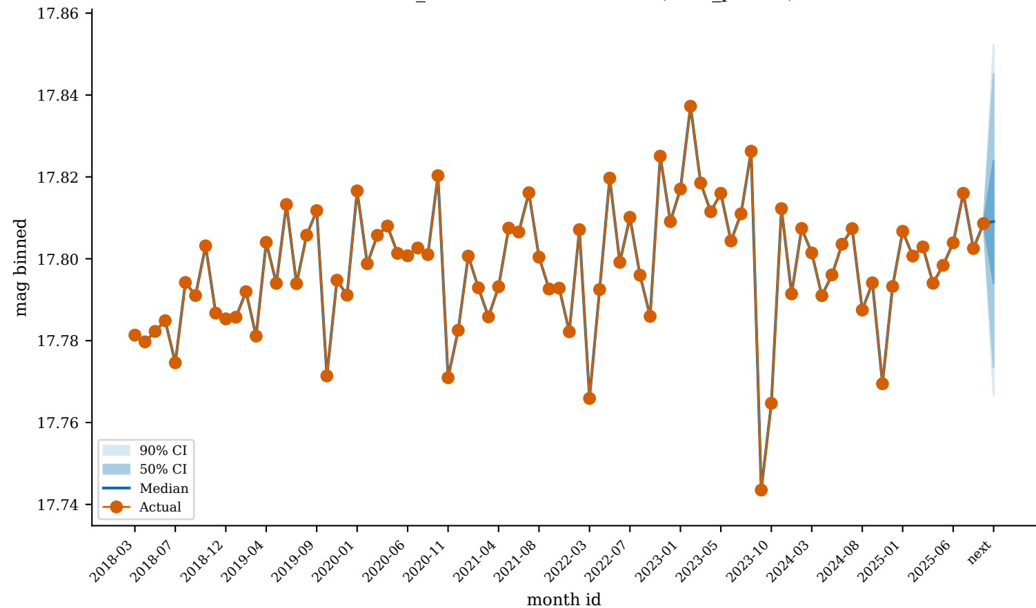
GaiaDR3_1714635091562696320 (most_prolific)
