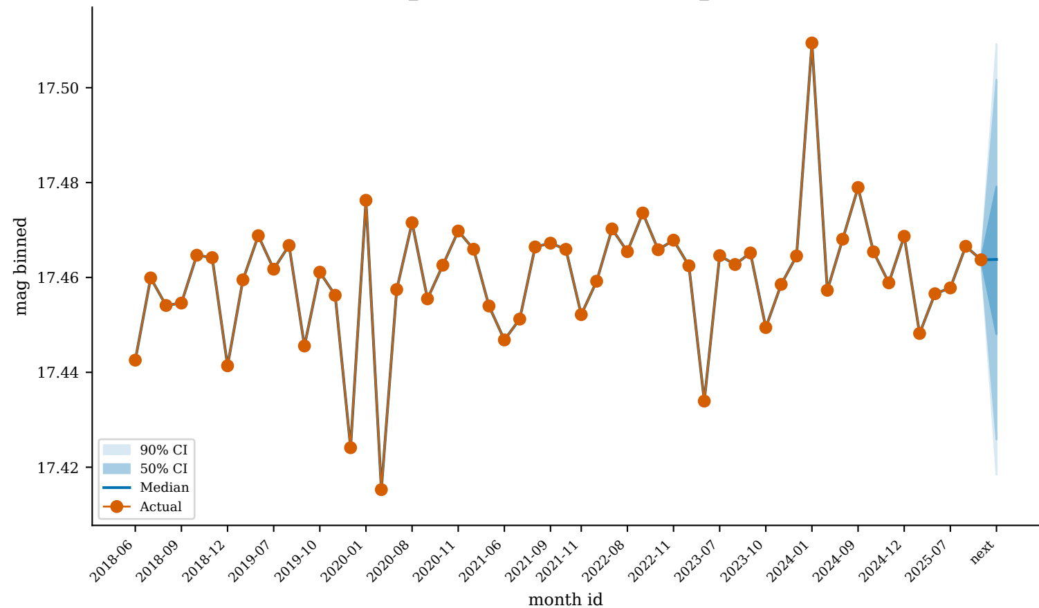
GaiaDR3_2543356006353057792 (best_predicted)
