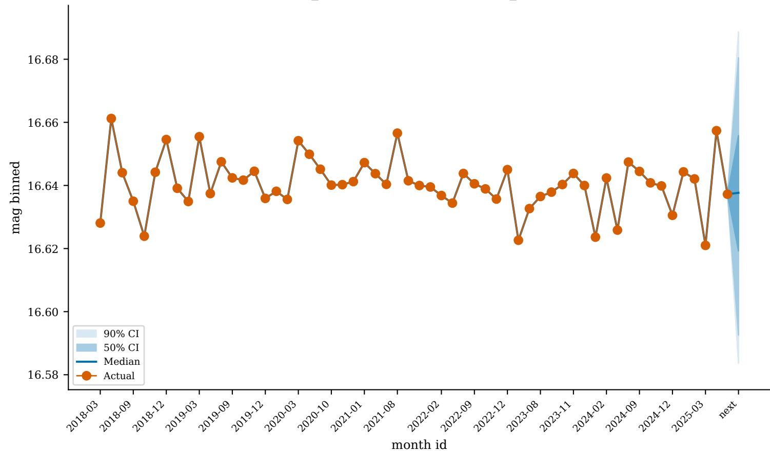
GaiaDR3_36207059639735296 (best_predicted)
