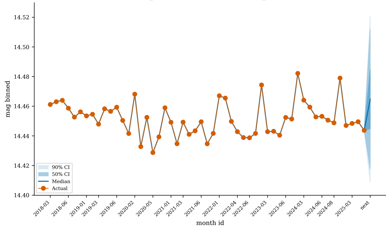
GaiaDR3_6332746557159637504 (worst_predicted)
