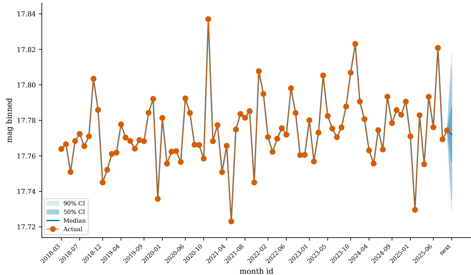
GaiaDR3_1430581420783430528 (most_prolific)
