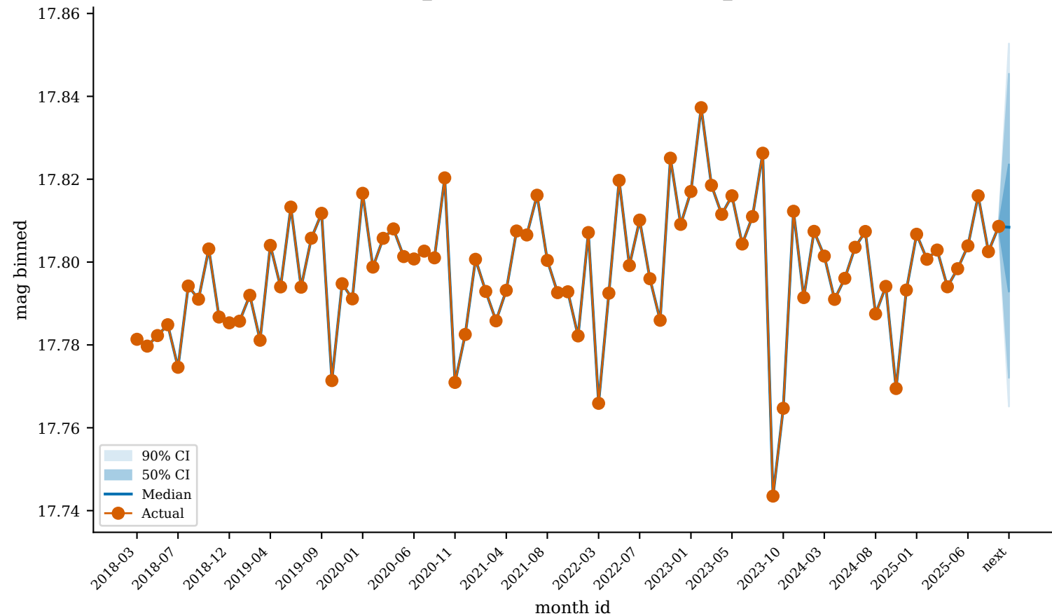
GaiaDR3_1714635091562696320 (most_prolific)
