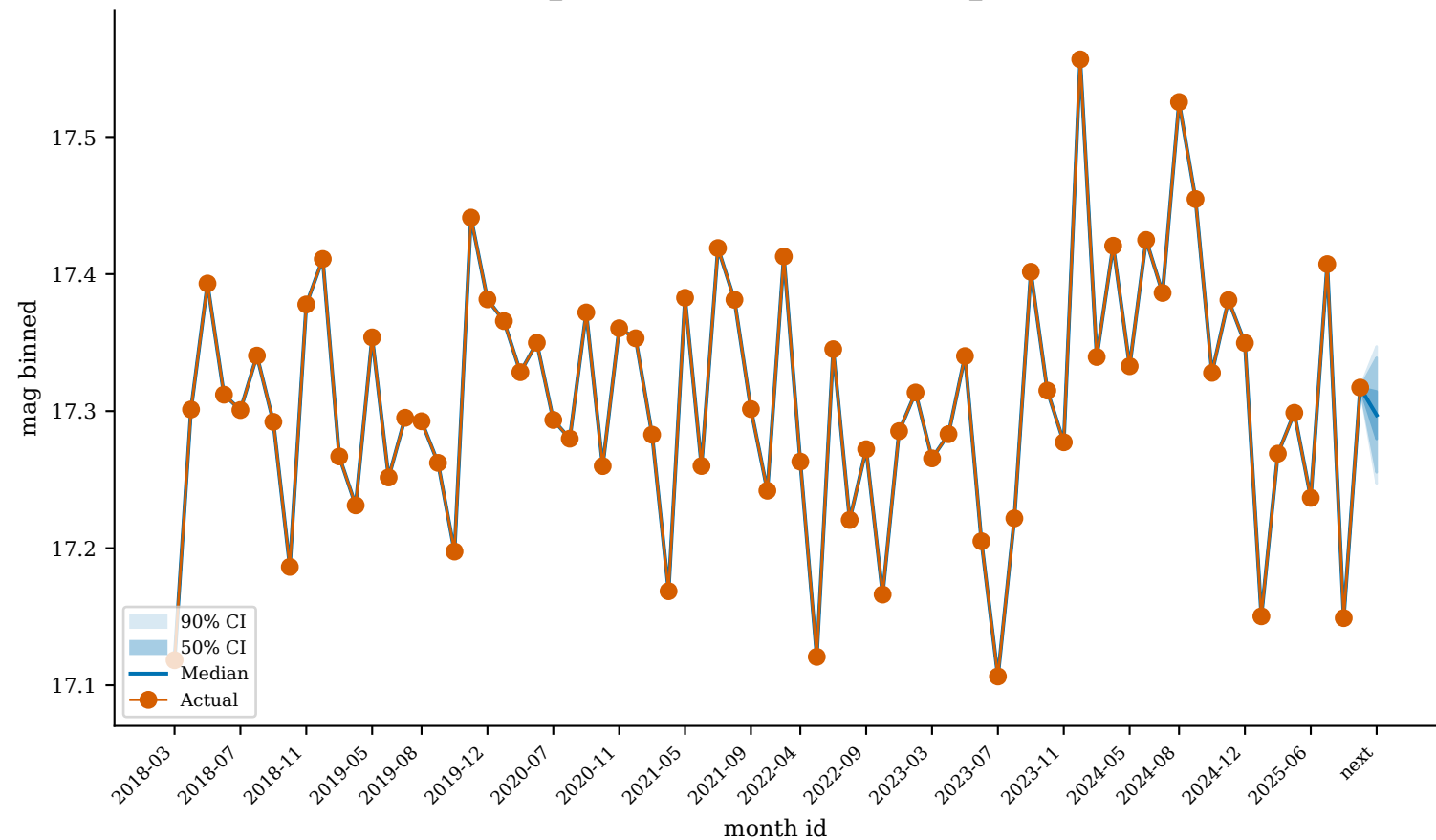
GaiaDR3_1863757043284422784 (worst_predicted)
