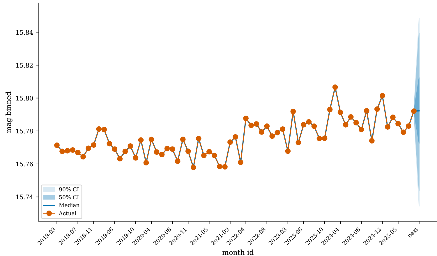
GaiaDR3_4322122179512445568 (best_predicted)
