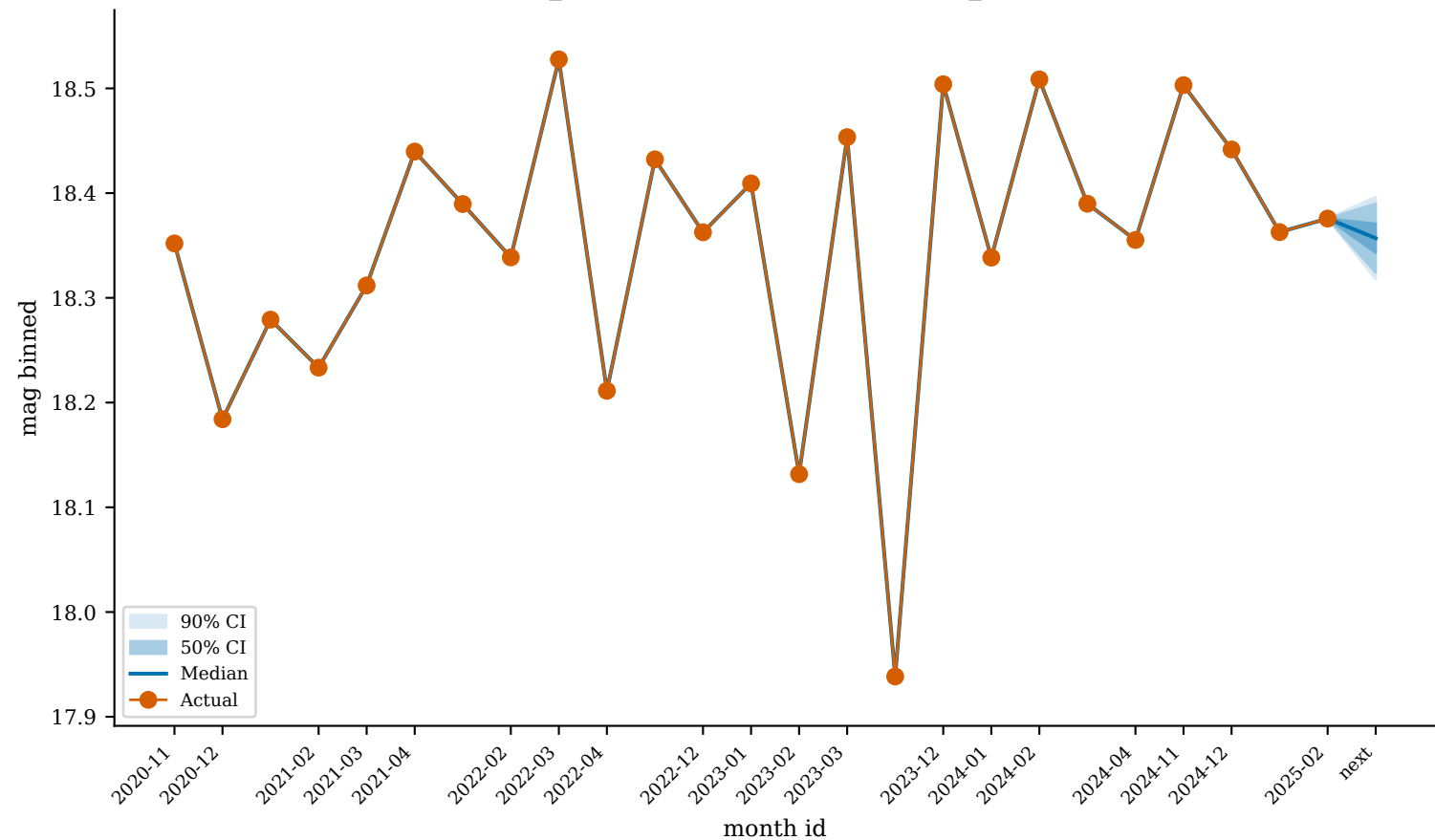
GaiaDR3_5645504991845223936 (worst_predicted)
