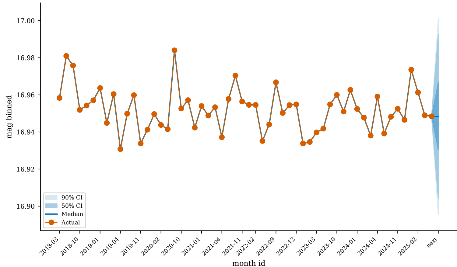
GaiaDR3_3102457123623043072 (best_predicted)
