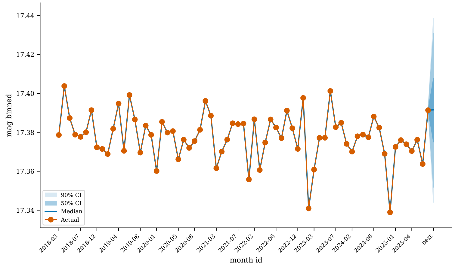
GaiaDR3_1188363918331170048 (best_predicted)
