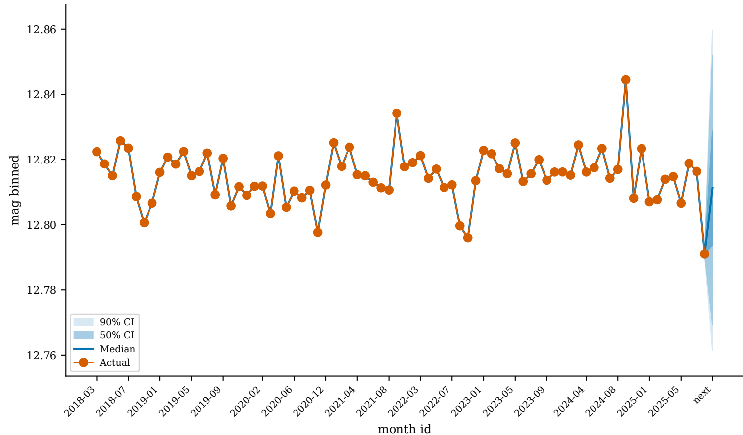
GaiaDR3_1504338718064197760 (worst_predicted)
