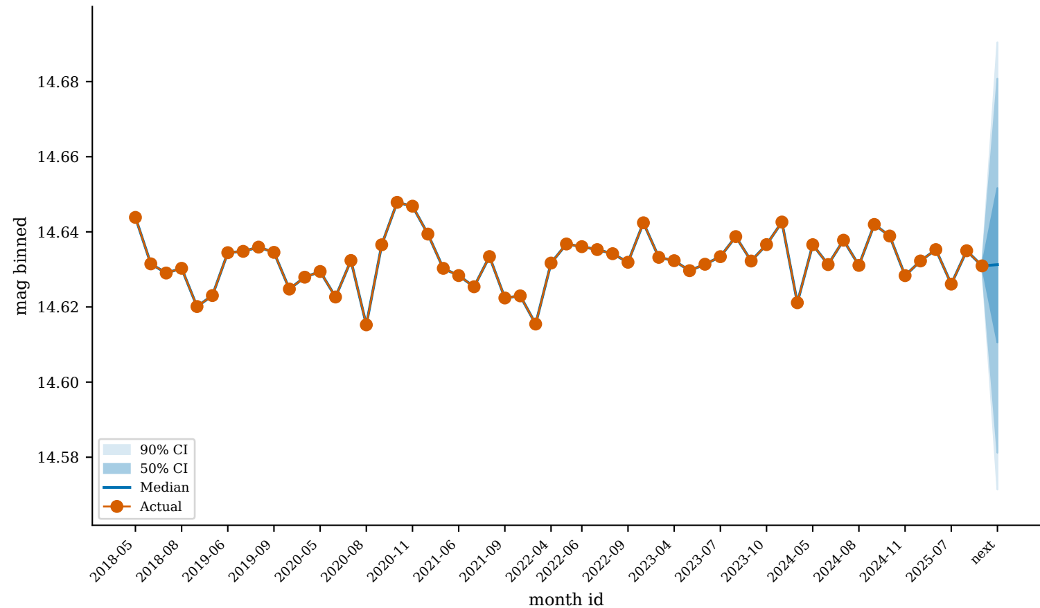
GaiaDR3_4181798519823760256 (high_uncertainty)
