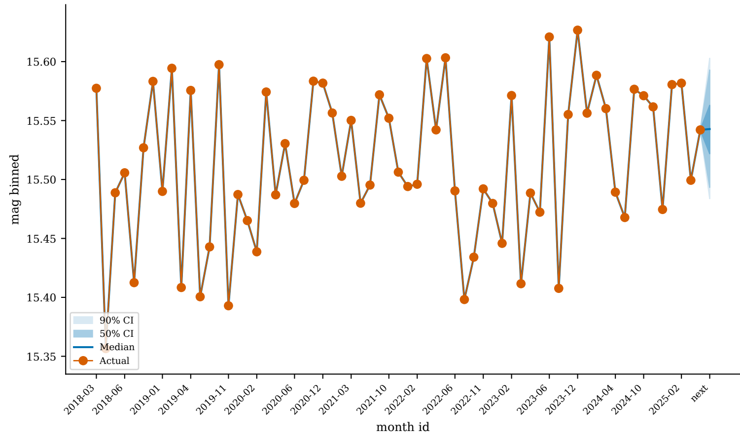
GaiaDR3_722446385752579840 (high_uncertainty)
