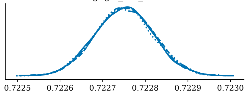
ztfgcgw_sigma_artist
