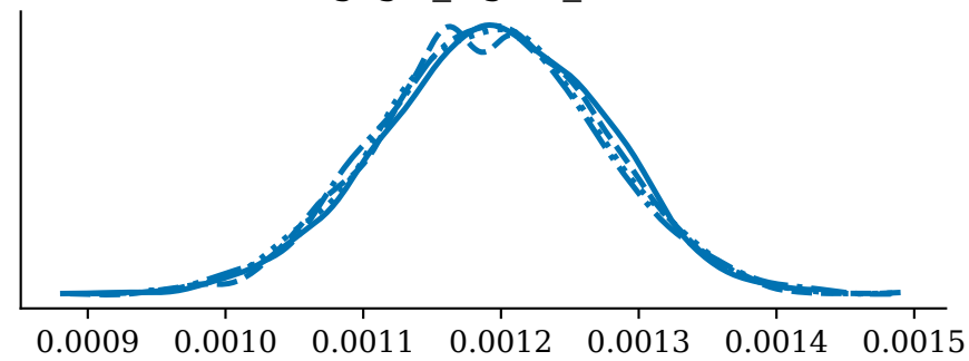
ztfgcgw_sigma_rw
