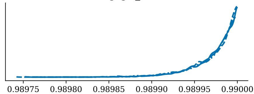
ztfgcgw_rho
