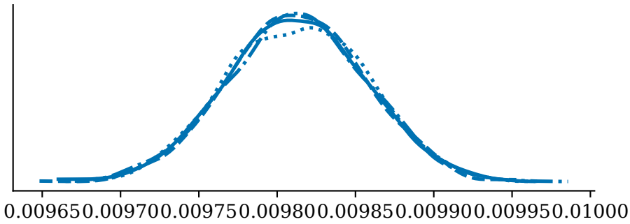
ztfgcgw_rho
