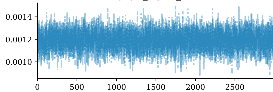
ztfgcgw_sigma_rw
