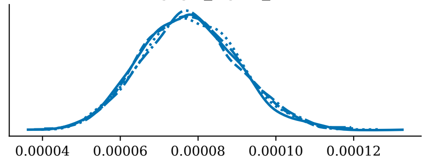
ztfgcgw_sigma_obs
