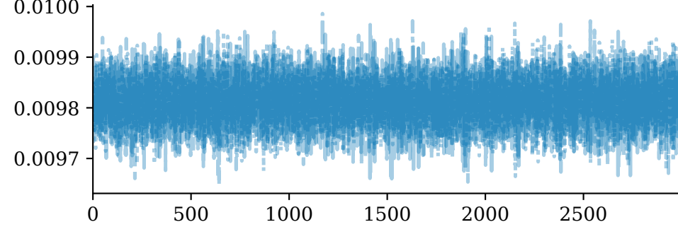
ztfgcgw_rho
