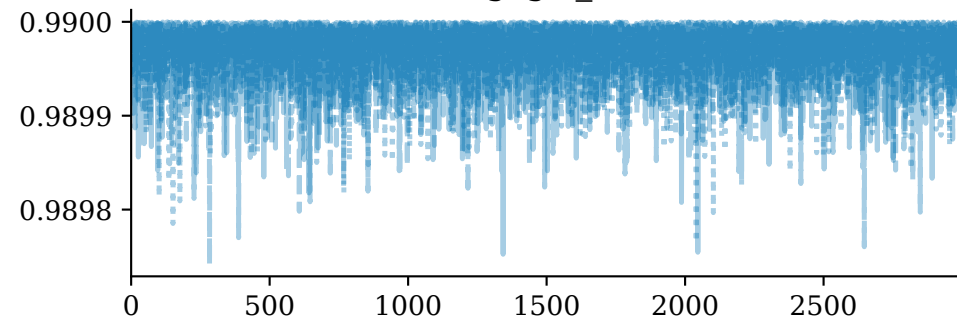
ztfgcgw_rho
