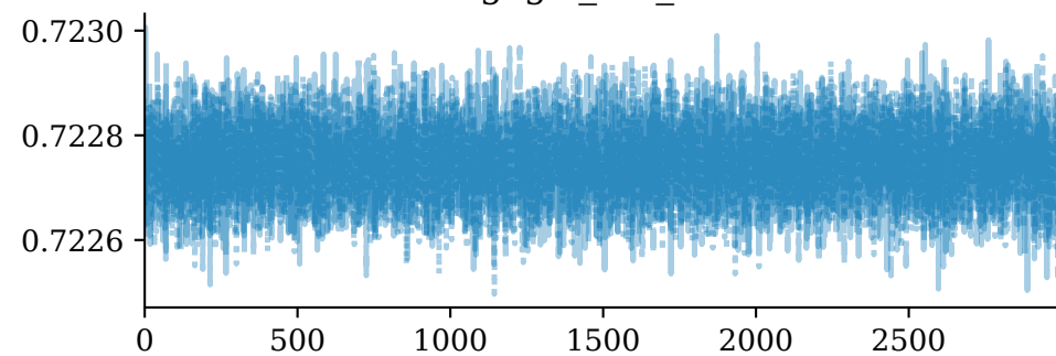
ztfgcgw_sigma_artist
