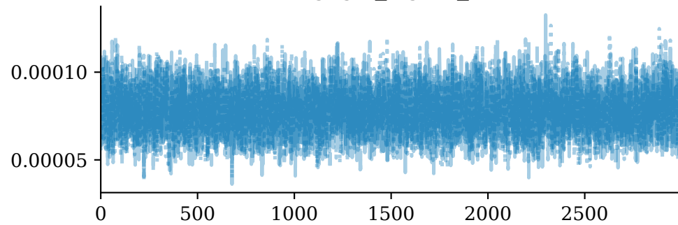
ztfgcgw_sigma_obs
