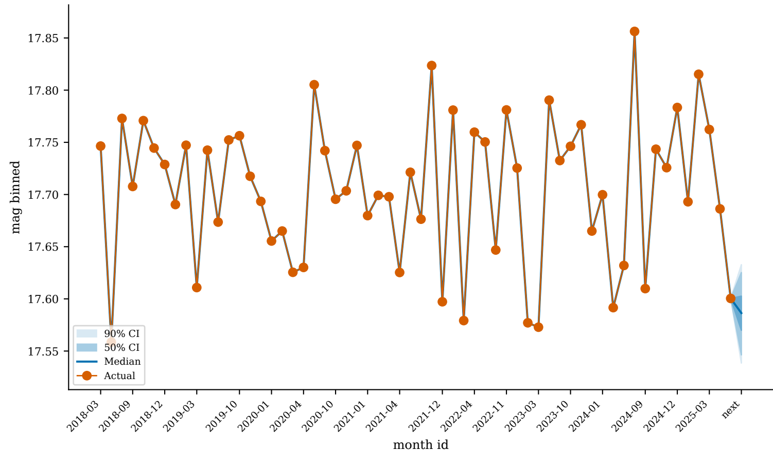
GaiaDR3_3345661467822106624 (worst_predicted)
