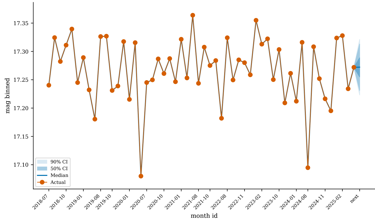
GaiaDR3_2498367529597482496 (best_predicted)
