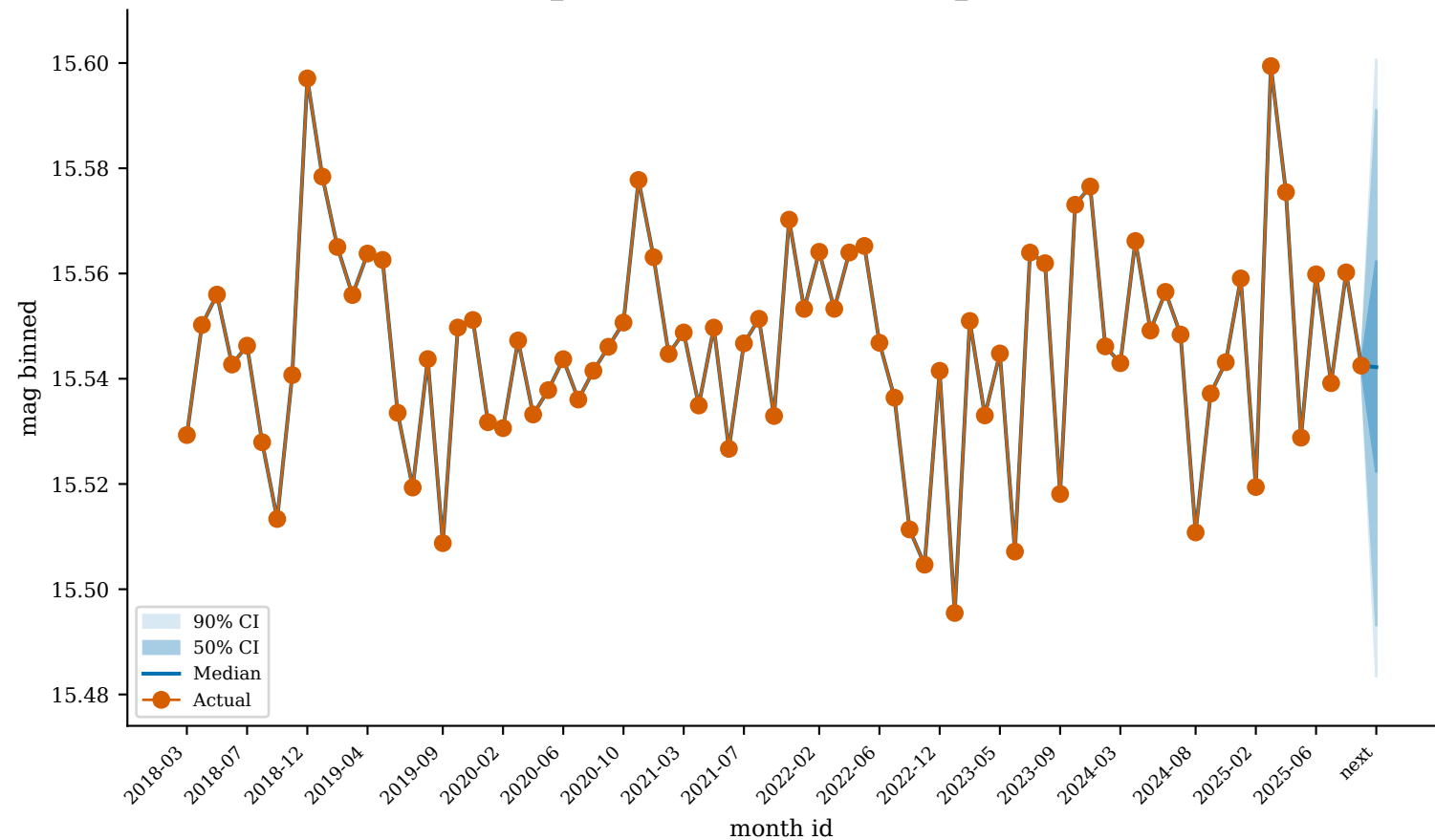
GaiaDR3_1641326979142898048 (high_uncertainty)
