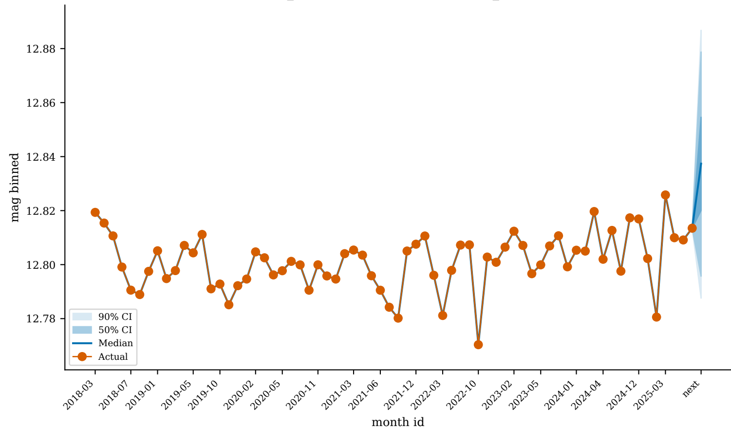
GaiaDR3_841336990381518208 (worst_predicted)
