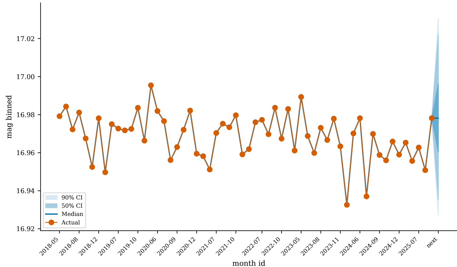
GaiaDR3_2674266437736332160 (best_predicted)
