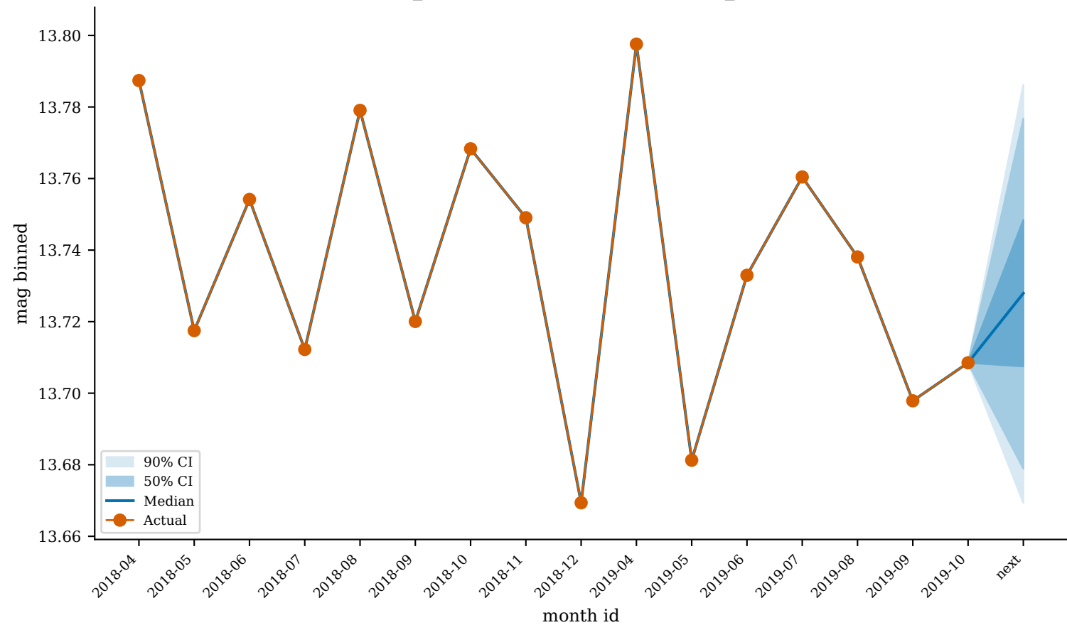
GaiaDR3_4235280071072332672 (worst_predicted)
