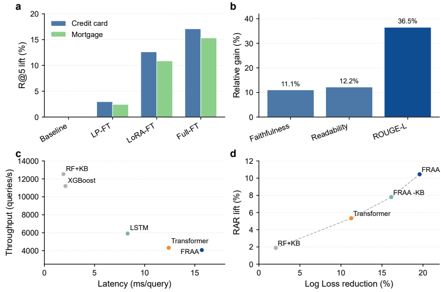
Fig. 4. Operational evaluation of FRAA. (a) Cross-scenario Recall@5 lift for credit-card and mortgage risk scenarios. (b) Relative explanation-quality gain over a template baseline. (c) Latency-throughput trade-off under the tested serving configuration. (d) Offline replay utility measured by risk-adjusted revenue lift against Log Loss reduction.
