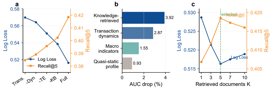
Fig. 3. Ablation and sensitivity analyses. (a) Component-level comparison of Log Loss and Recall@5 across the Transformer baseline, FRAA variants, and the full model. (b) Feature-family occlusion measured by AUC drop. (c) Retrieval-depth sensitivity, with K = 5 selected for the main experiments.
