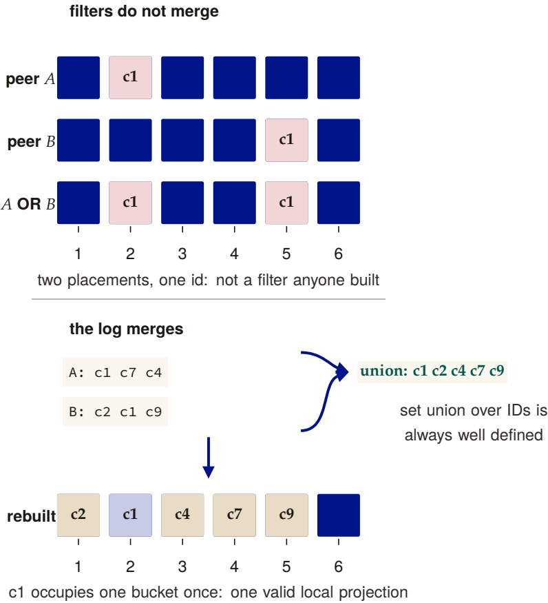
Figure 2.5: Two six-bucket cuckoo filters compared before and after the design change. Top: peer A inserts c1 into bucket 2 and peer B inserts the same c1 into bucket 5, an artifact of each peer’s own insertion and eviction history; bitwise OR keeps both placements, which is a state no single filter build could have produced. Bottom: gossiping the append-only ID log instead—peer A’s c1 c7 c4 and peer B’s c2 c1 c9—and taking the ordinary set union gives c1 c2 c4 c7 c9; each daemon rebuilds one local filter with c1 in a single bucket. [internal]
