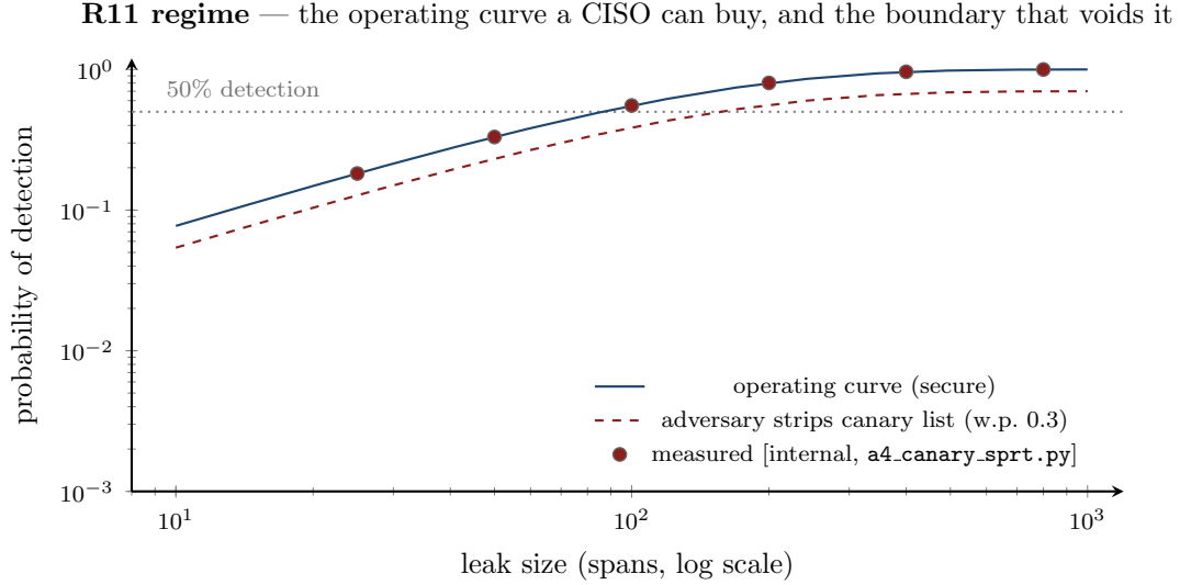
Figure 5: Regime diagram for Pillar IV: the operating curve a CISO can buy, and the boundary that voids it. Left: \Pr(\text{detect}) against leak size m at density 1%, \beta = 0.2 — exact, approximate, and simulated agree [internal, a4_canary_sprt.py ]. The guarantee’s load-bearing regime is secret, uniform planting: an adversary who obtains the canary list with probability 0.3 and strips all of them drops measured power from 0.9997 to 0.698 at k=5 [internal].
