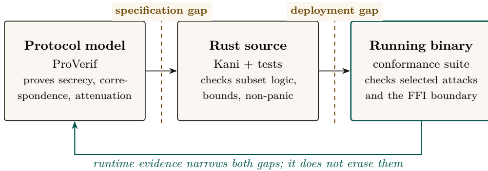
Figure 8: Assurance crosses two explicit gaps: a verified protocol model is not automatically the Rust implementation, and verified source is not automatically the deployed binary. Runtime evidence flows back across the same boundaries without turning either assumption into a theorem.
